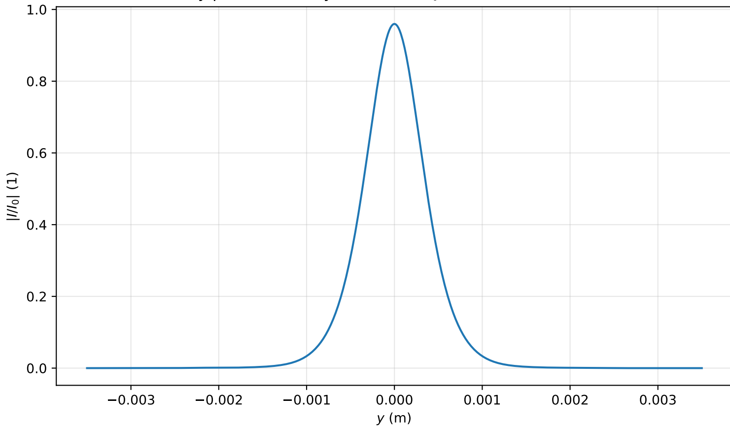
Intensity profile I(x = 0, y, z = 3.582)/I_0 , P_{in}=0.8P_{cr} , artificial time
